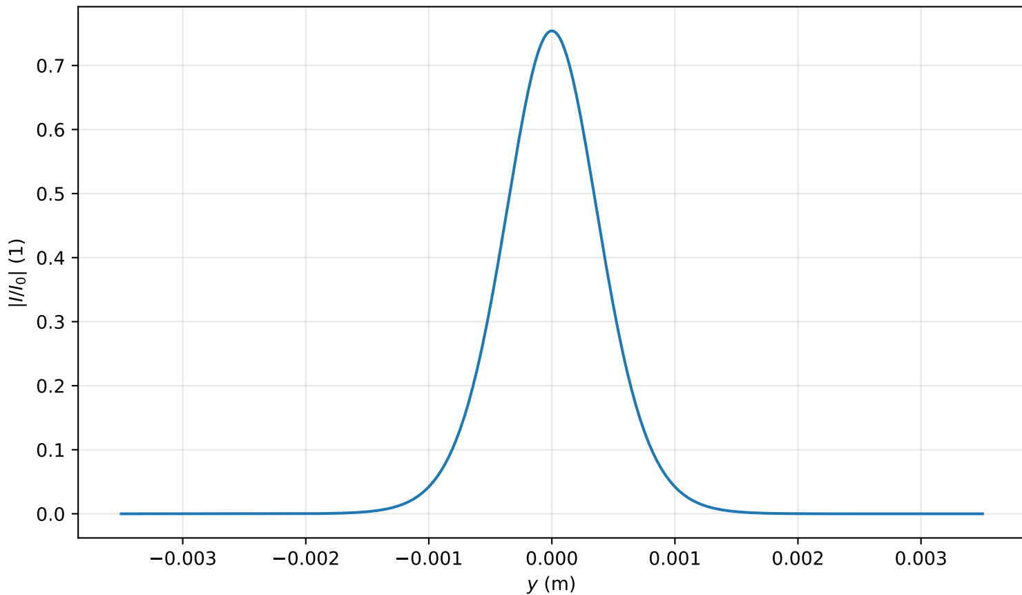
Intensity profile I(x=0, y, z=1.911)/I_0 , P_{in}=0.4P_{cr} , artificial time
